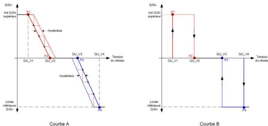
figure 8-4 Courbe Q(U)
