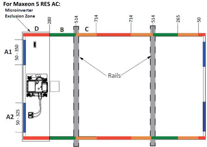
Fig.1 With Rail Support
